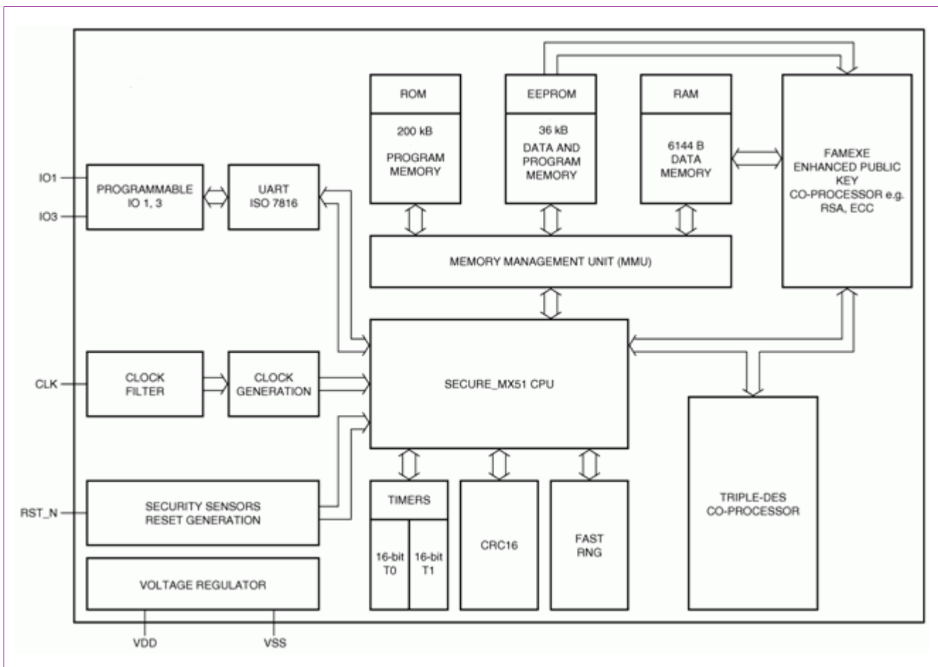
Fig 1. Block Diagram of the P5CC037V0A
