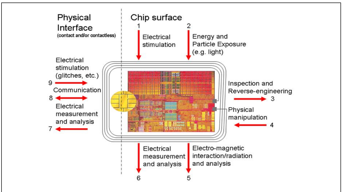
Figure 3-3 Interactions between the TOE and its outer world
