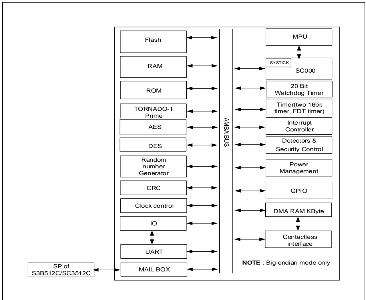
Figure 1-1 S3B512C/SC3512C Block Diagram
