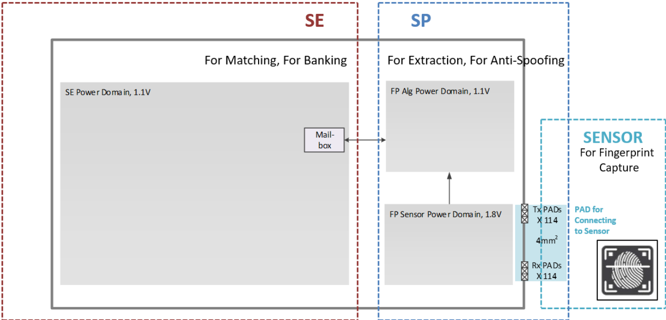
Figure 1-2 S3B512C/SC3512C Architecture
