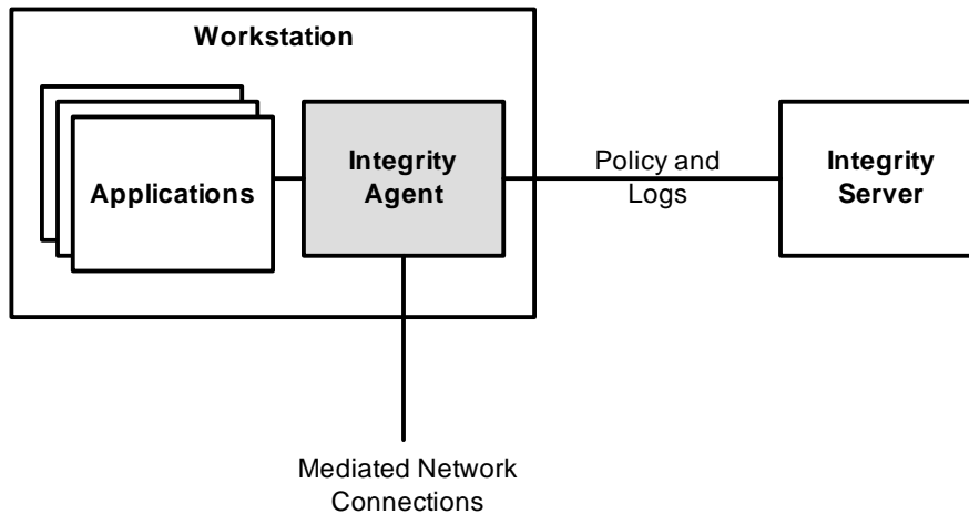
Figure 1 - TOE Configuration
