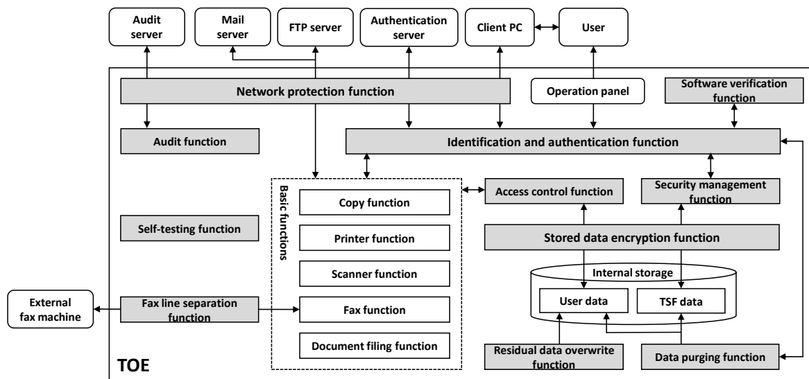
Figure 5-1 TOE boundary
