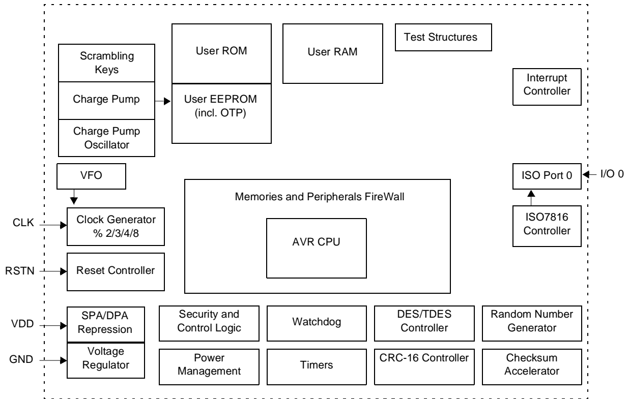
Figure 2-1 AT90SC6404R Block Diagram
