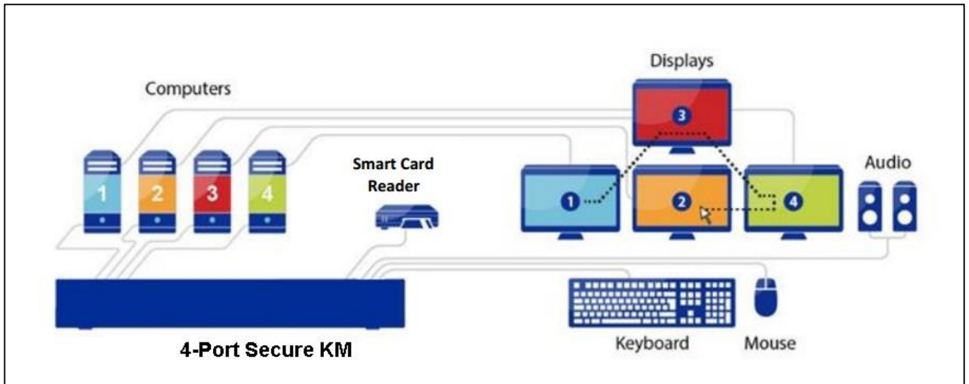
Figure 2 – Typical example of Vertiv Cybex 4-Port Secure KM Switch TOE installation
