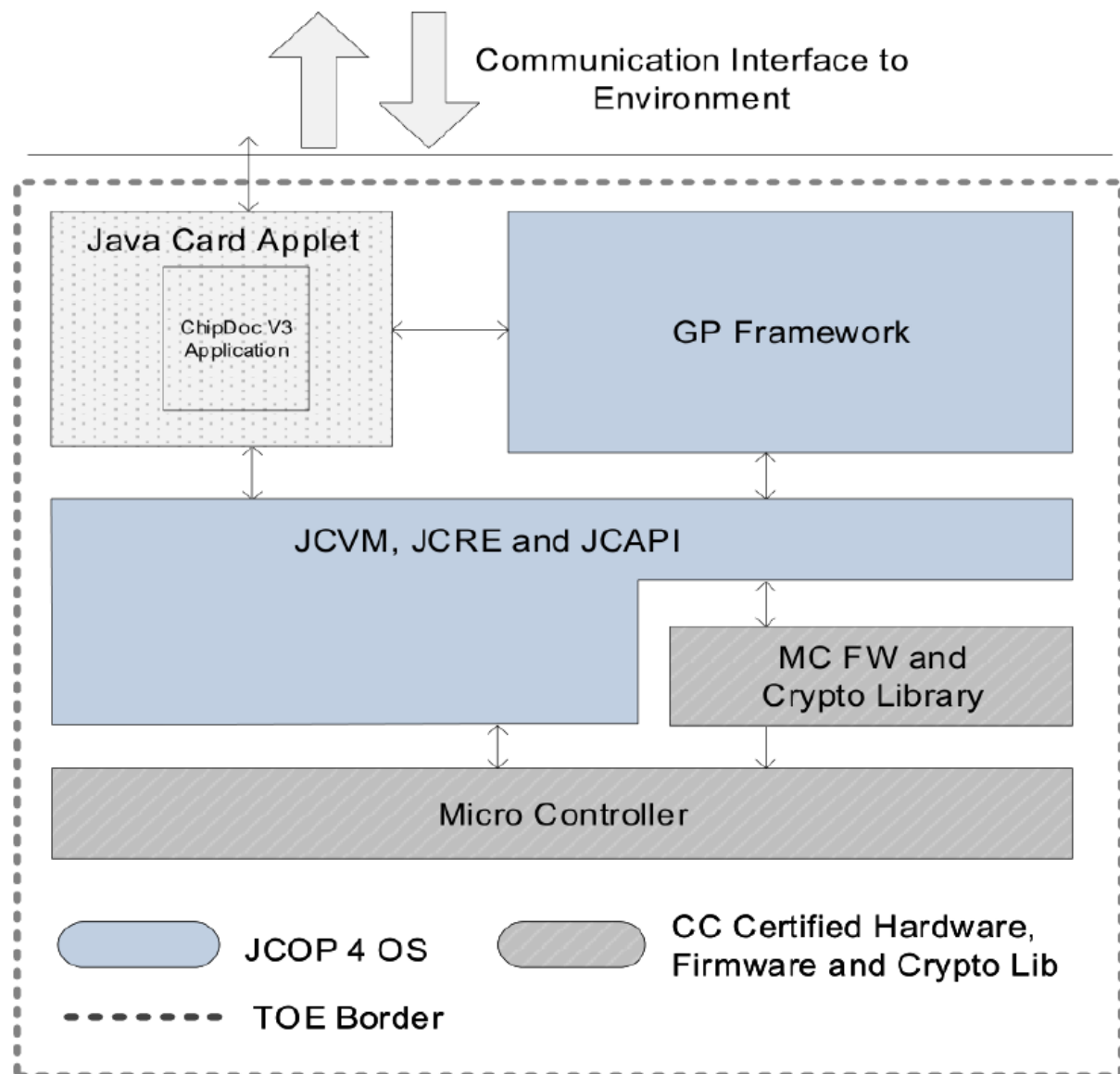
Figure 1. Architecture
