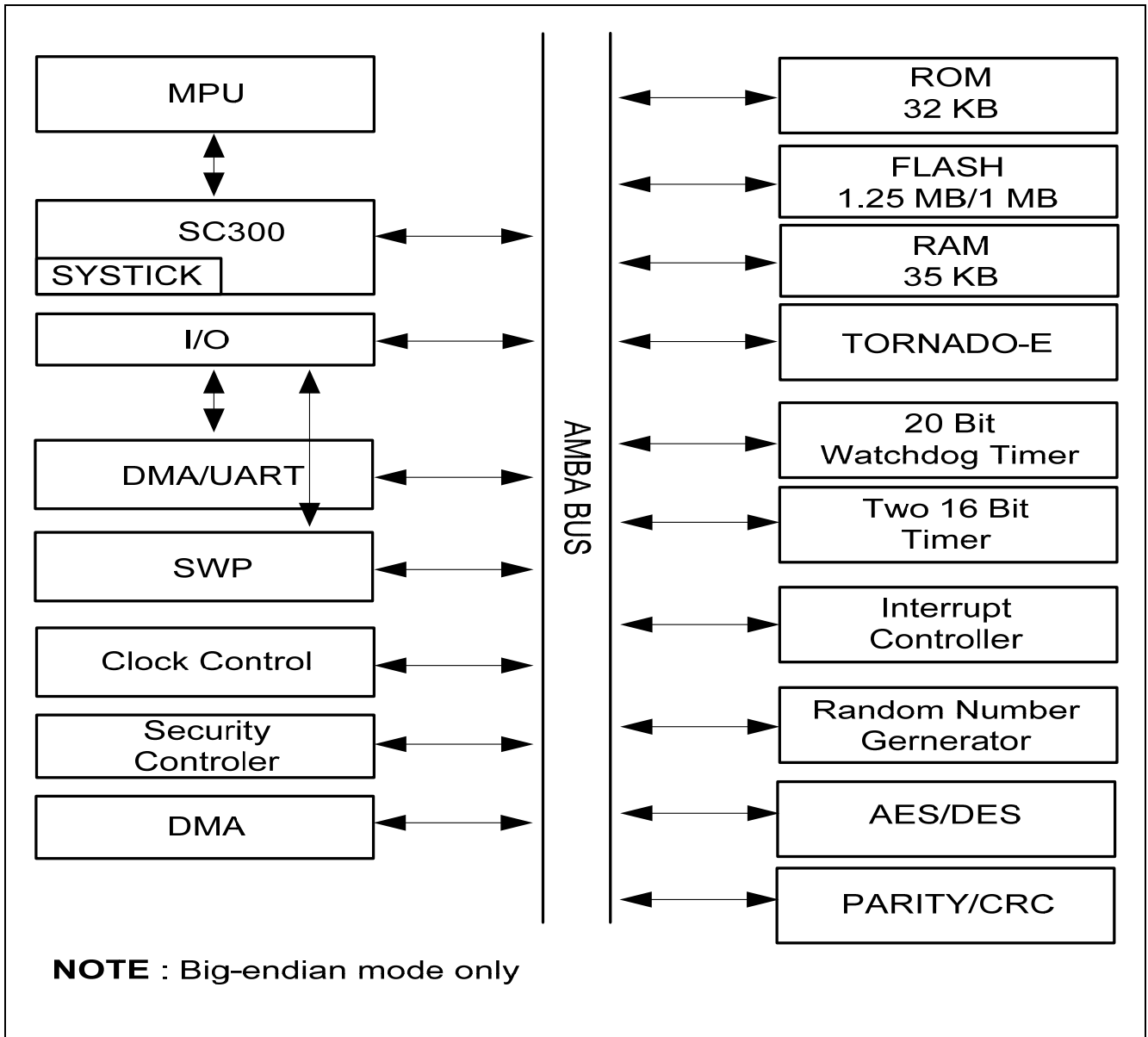
Figure 1. S3FV9QM/S3FV9QK Block Diagram
