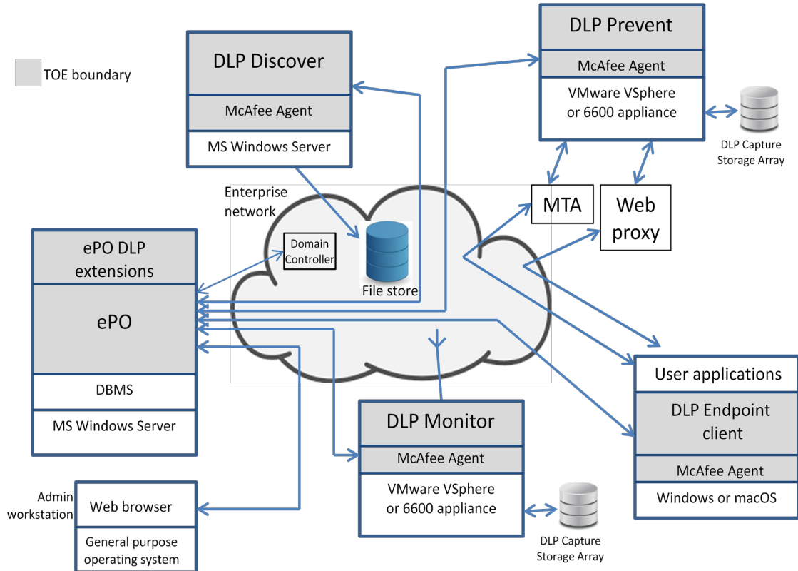
Figure 2 – Scope of the TOE
