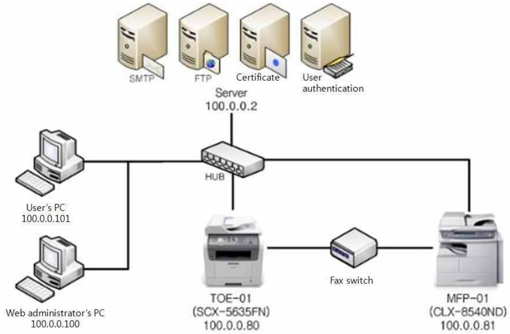
[Figure 3] Evaluator test configuration
