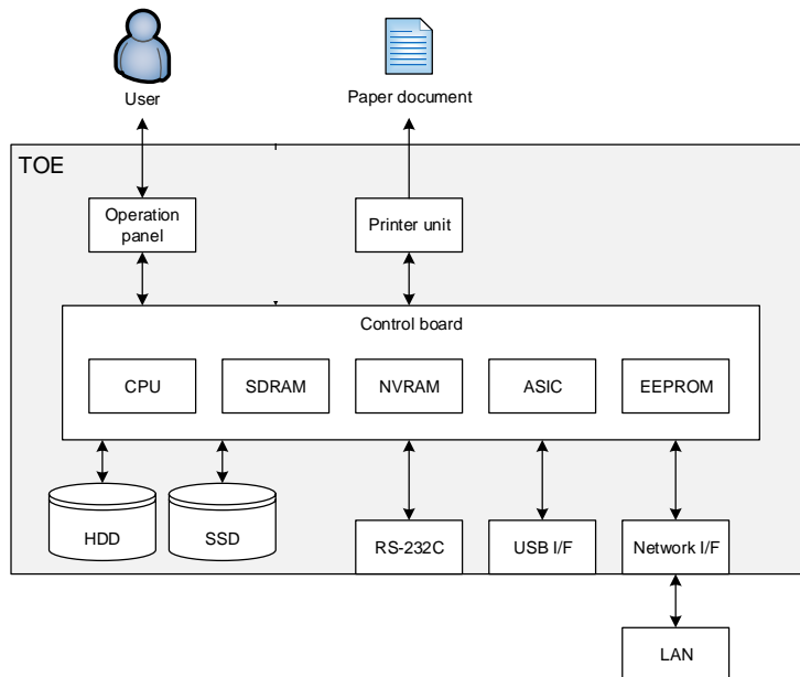
Figure 1-2 Physical scope of TOE
