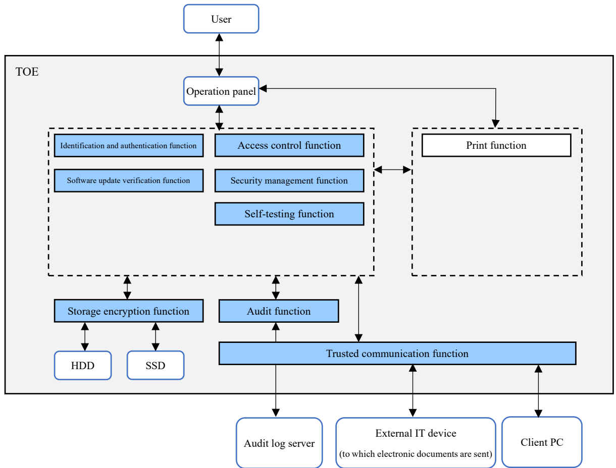
Figure 1-3 Logical scope of TOE
