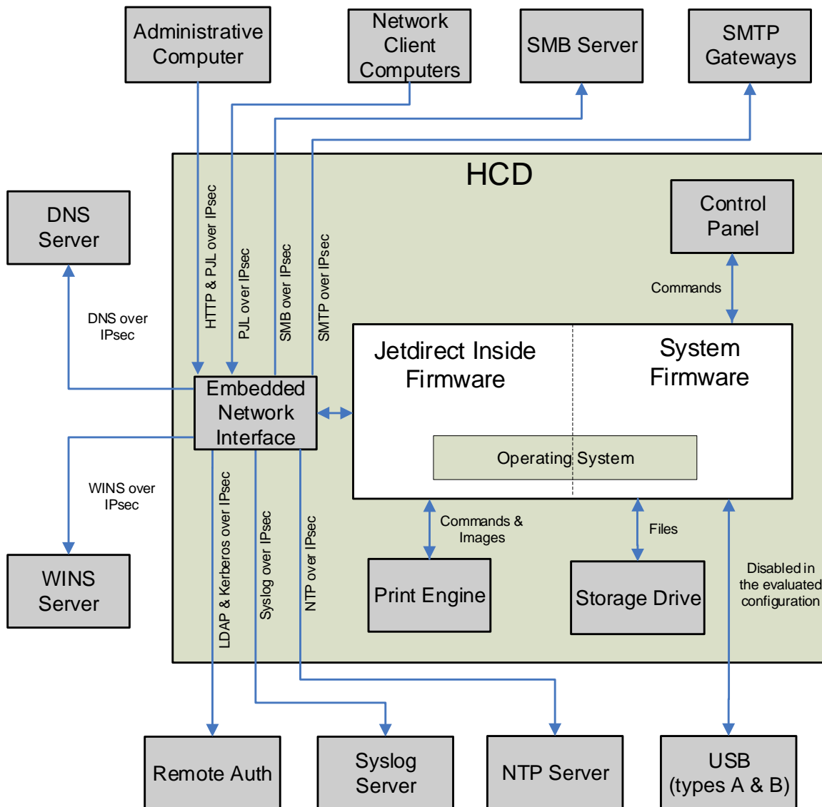
Figure 1 shows a high-level physical diagram of an HCD with the unshaded areas representing the TOE and the shaded areas indicating components that are part of the Operational Environment.
