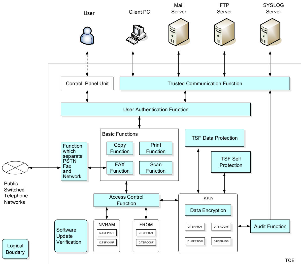
Figure 2 Logical Boundary
