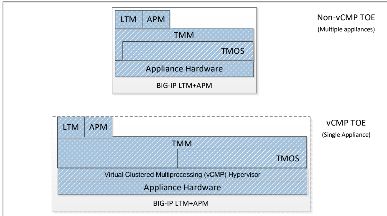
Figure 2: BIG-IP Subsystems
