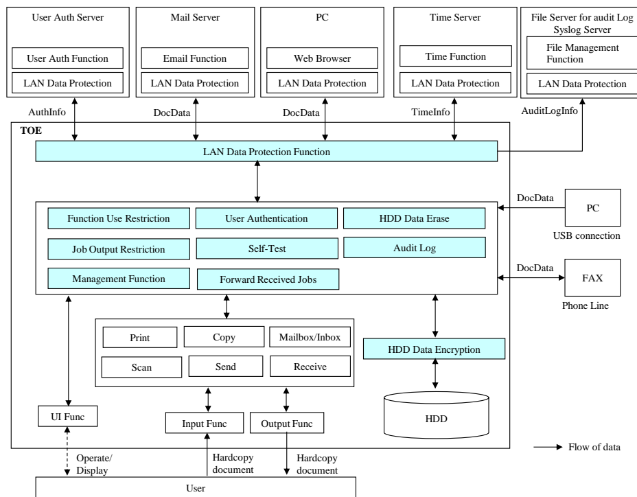
Figure 5-1 TOE Boundary
