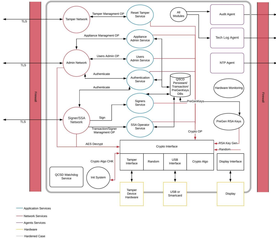
Figure 1. Logical architecture of the TOE
