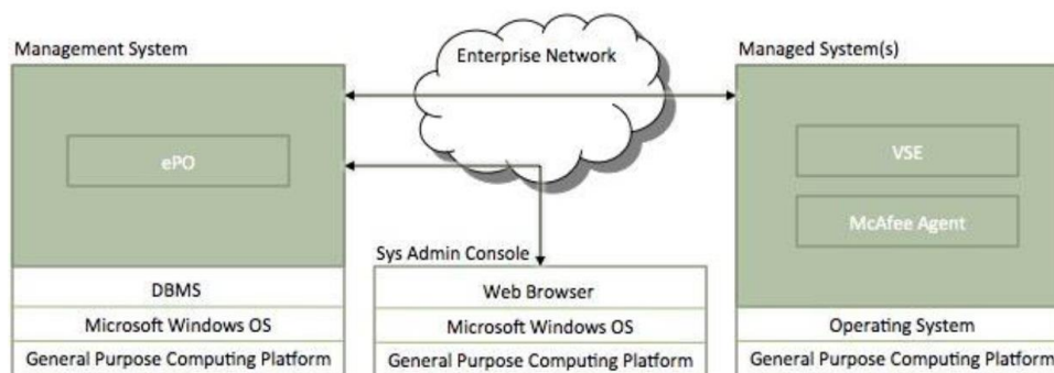
Figure 1 TOE Architecture
