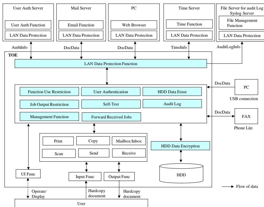
Figure 5-1 TOE Boundary
