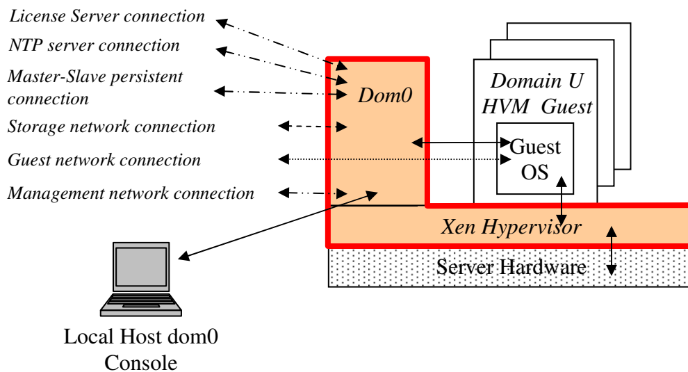
Figure 2 - TOE Architecture
