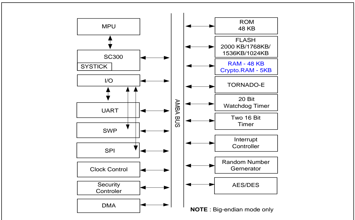
Figure 1 S3FV9RR/S3FV9RQ/S3FV9RP/S3FV9RK Block Diagram
