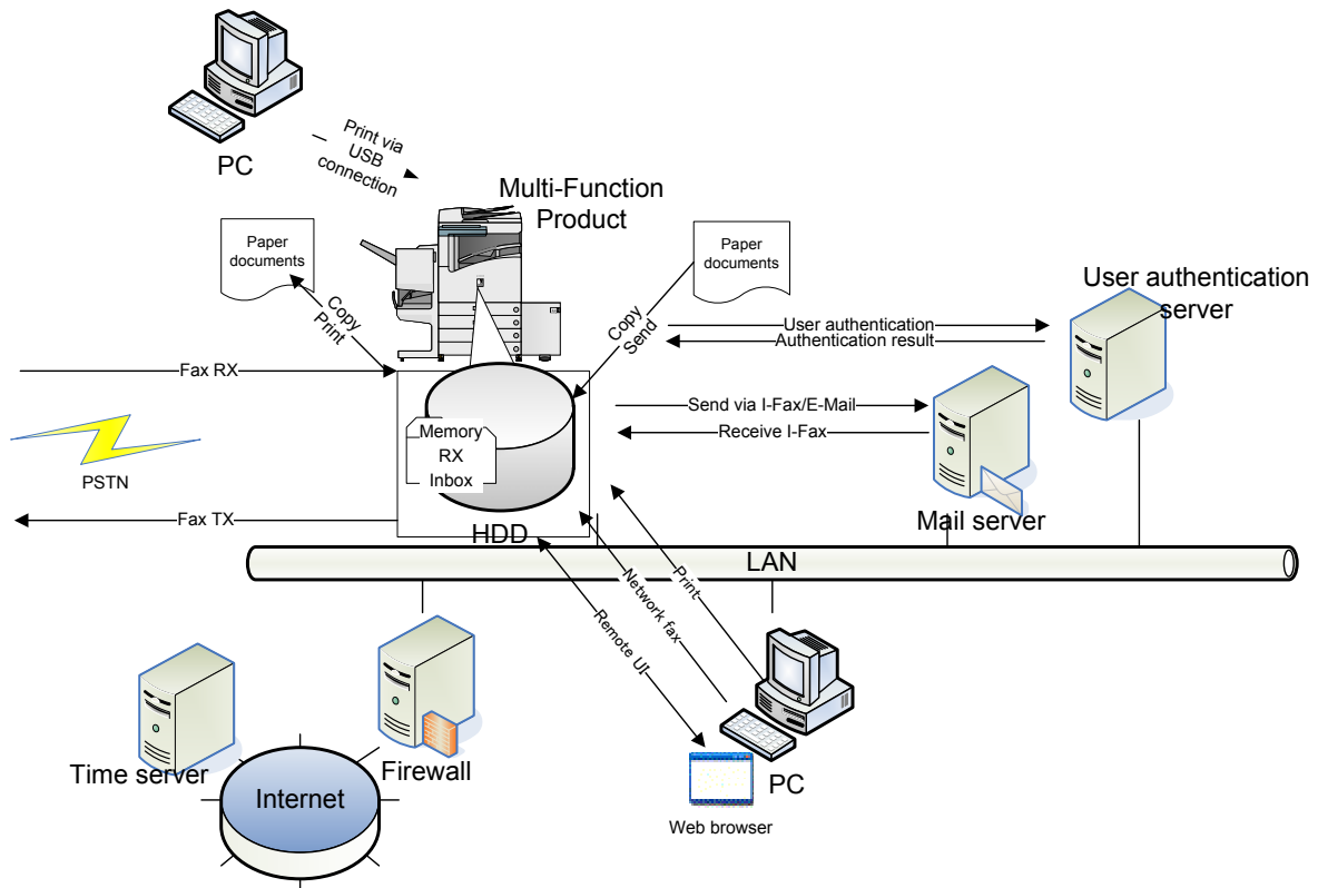
Figure 1 The assumed operational environment of the MFP < Canon imageRUNNER ADVANCE 500/400 Series >
