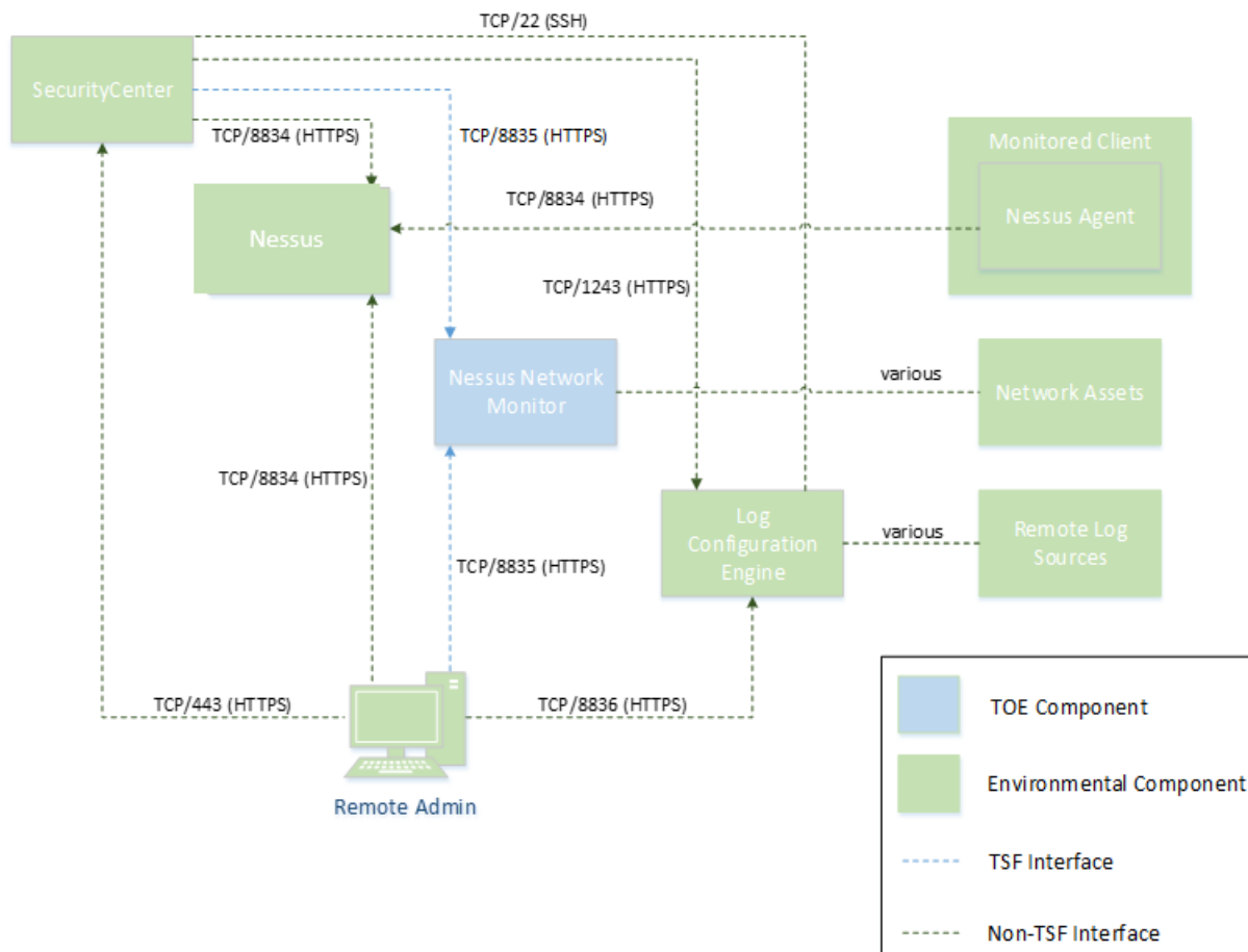
Figure 1 - TOE Boundary
