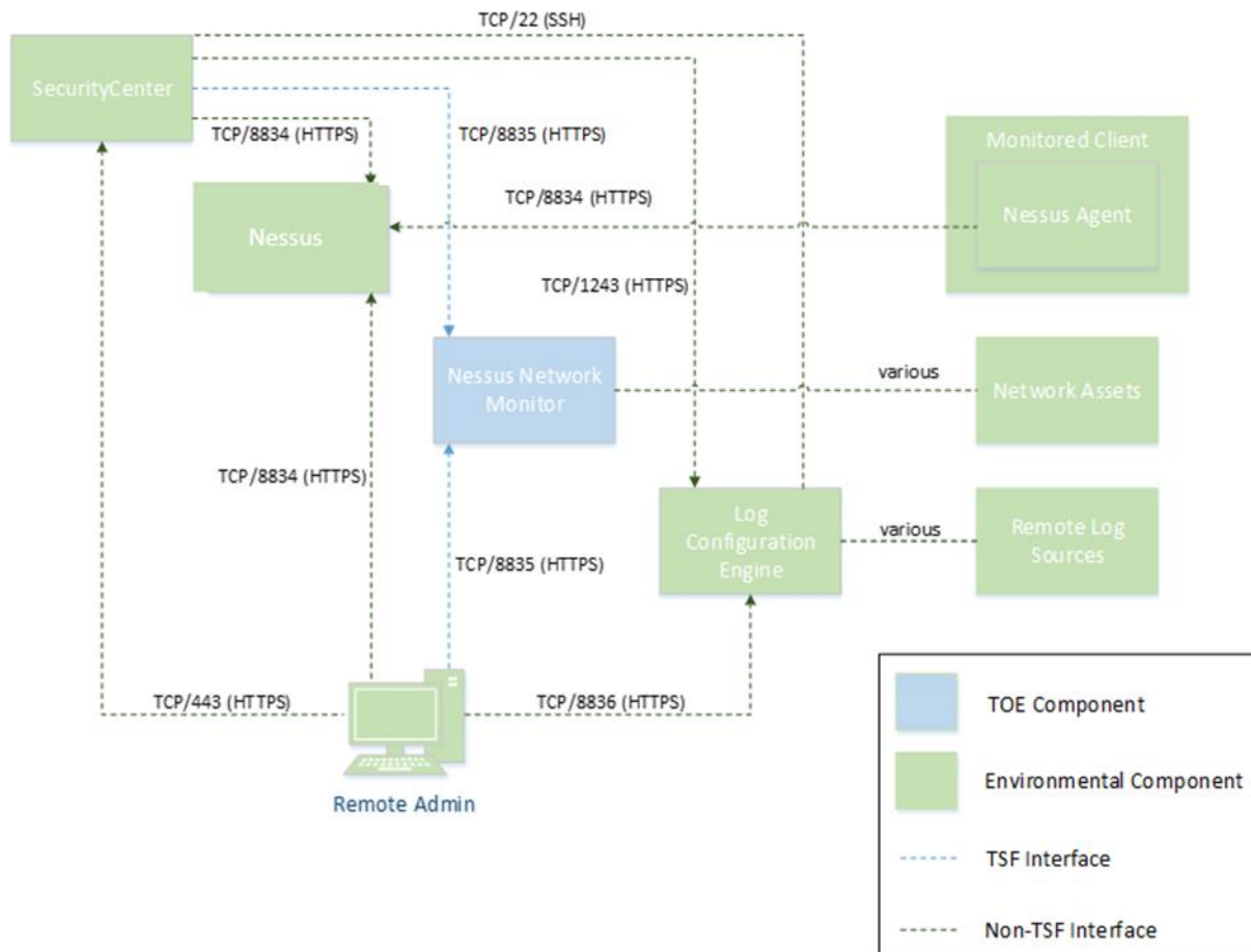
Figure 1: Nessus Network Monitor 6.2.2 Architecture
