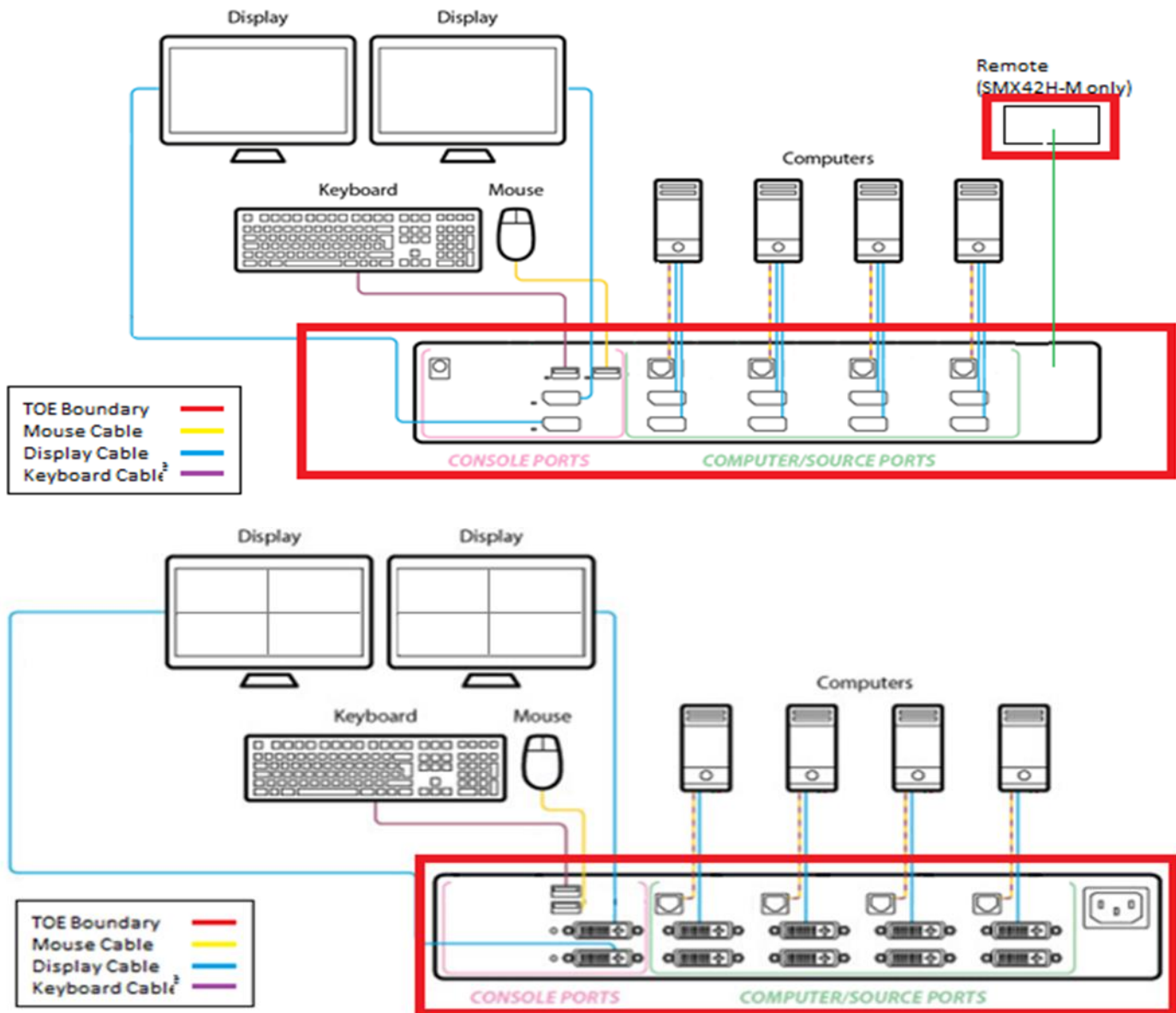
Figure 1: TOE Architecture
