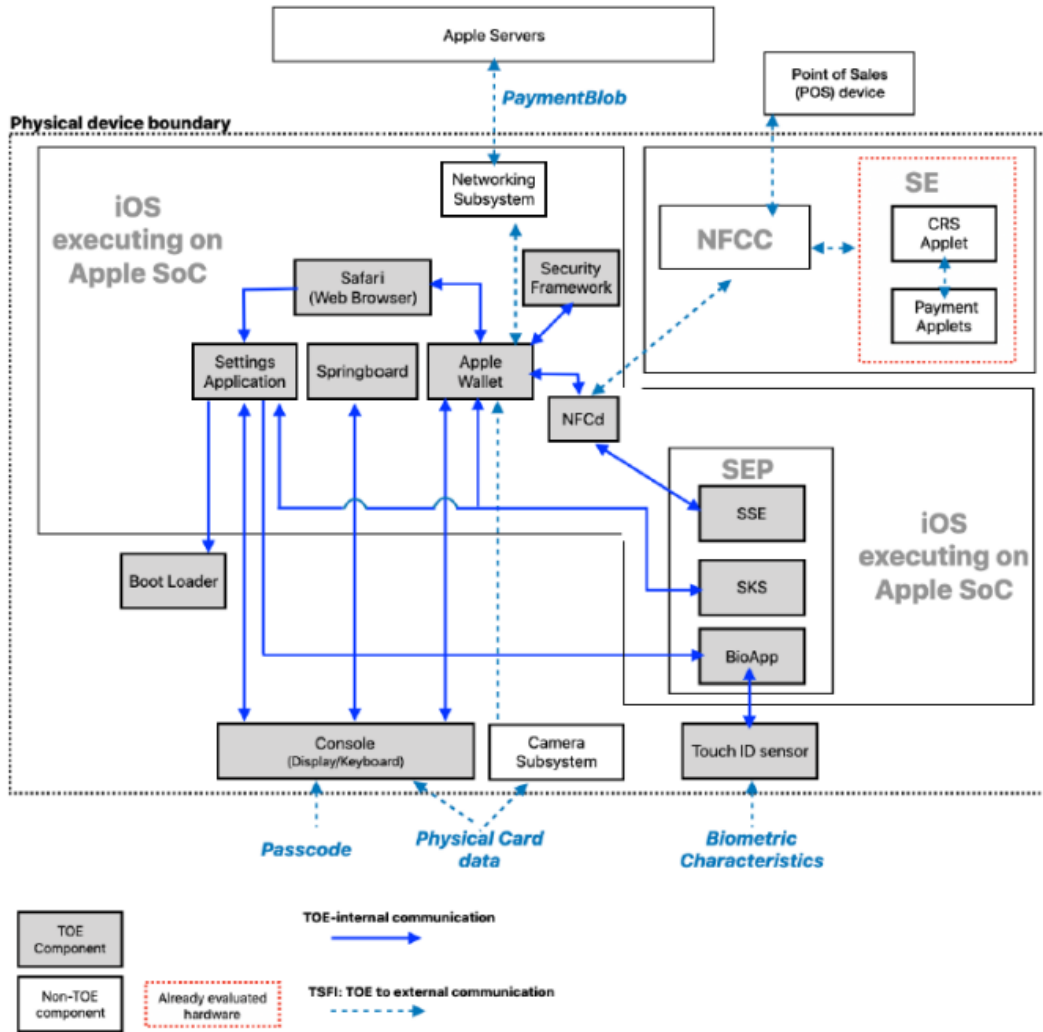
Figure 1: Product Architecture
