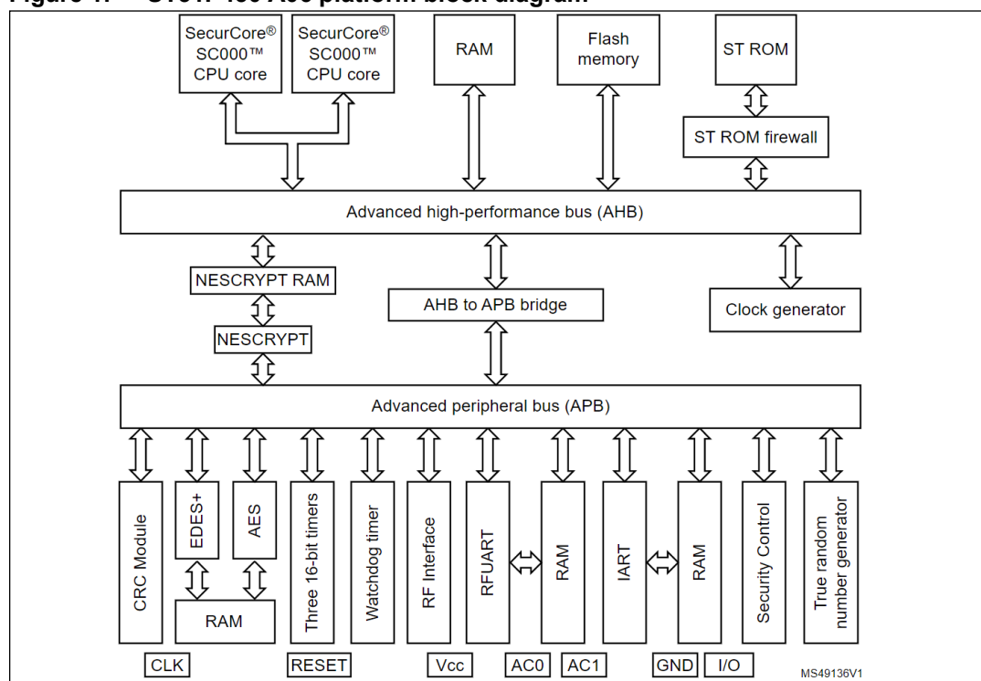
Figure 1. ST31P450 A06 platform block diagram
