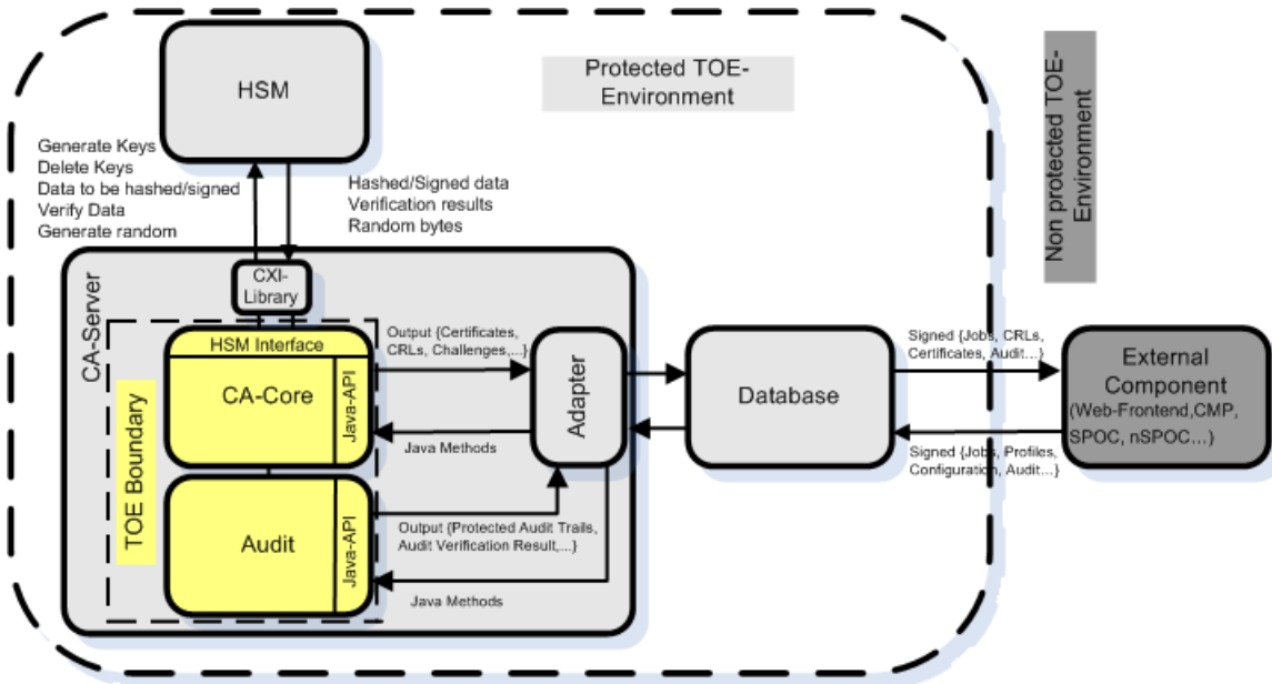
Figure 1: TOE boundary
