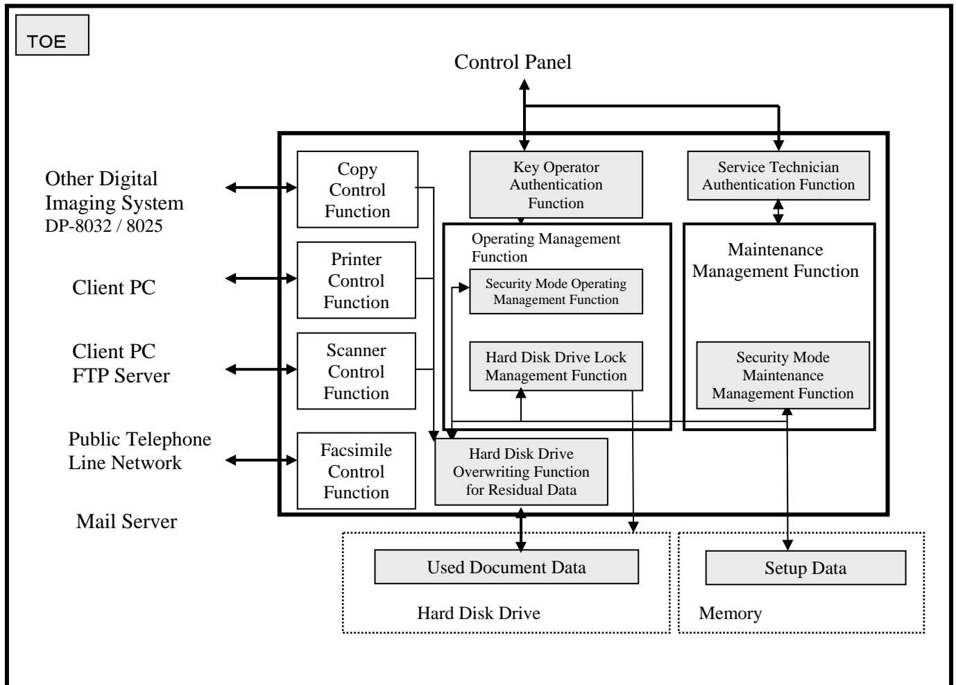
Fig. 3 Logical Configuration of Digital Imaging System DP-8032 / 8025 and TOE
