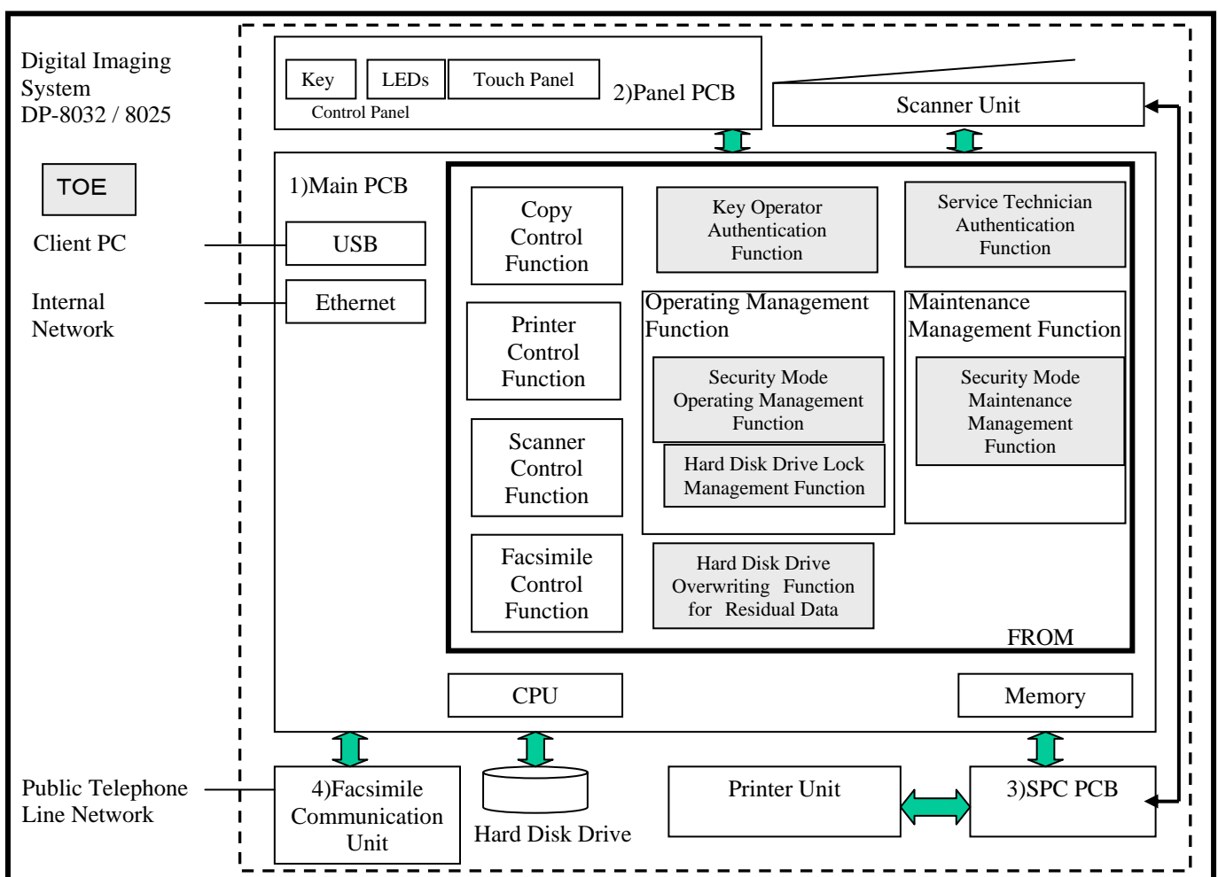
Fig. 2 Physical Configuration of Digital Imaging System DP-8032 / 8025 and TOE
