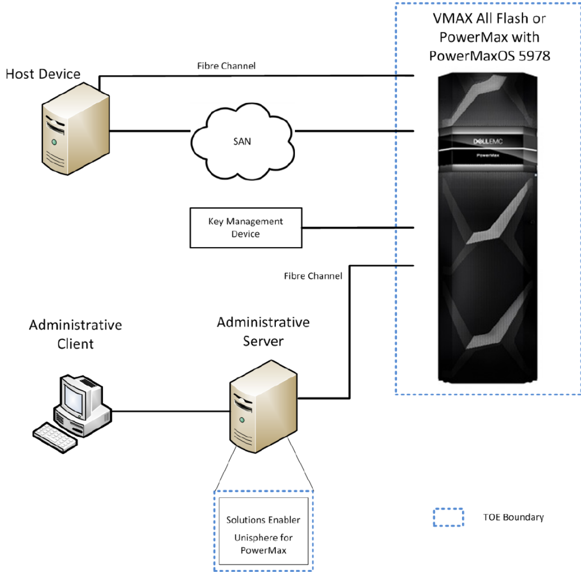
Figure 1 TOE Architecture
