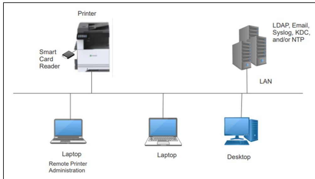
Figure 1: TOE Architecture
