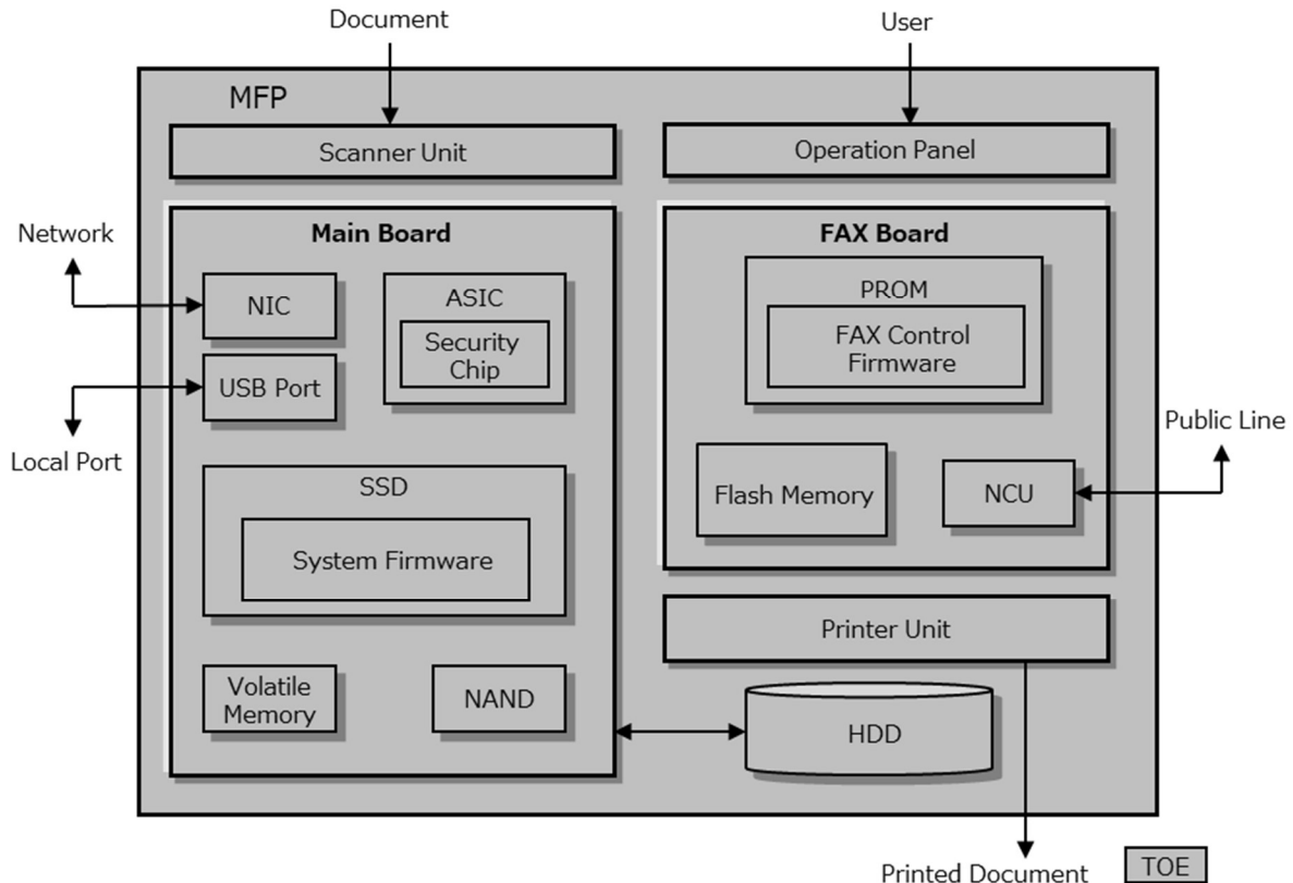
Figure 1 Physical Configuration of TOE
