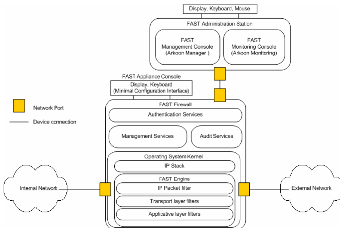
Figure 2 - Architecture du pare-feu
