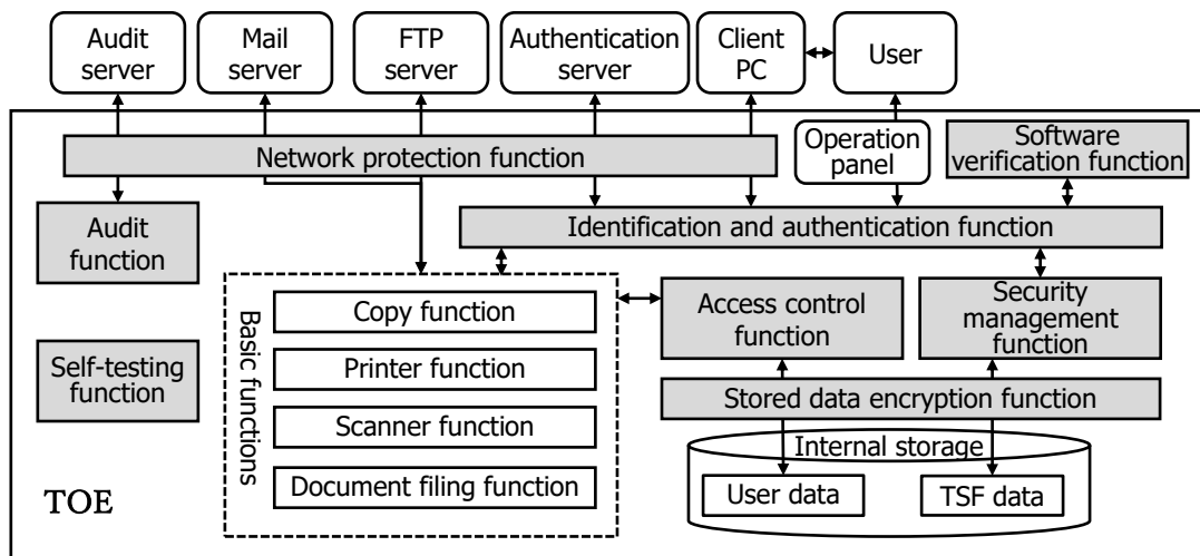
Figure 5-1 TOE boundary
