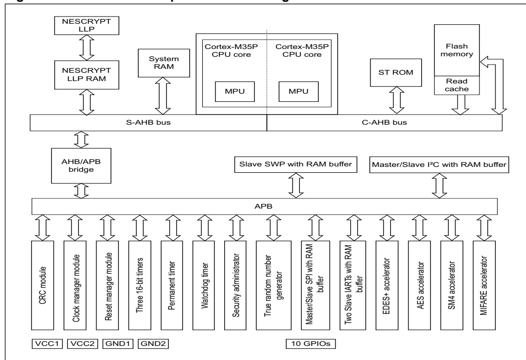
Figure 1. ST31N600 A02 platform block diagram
