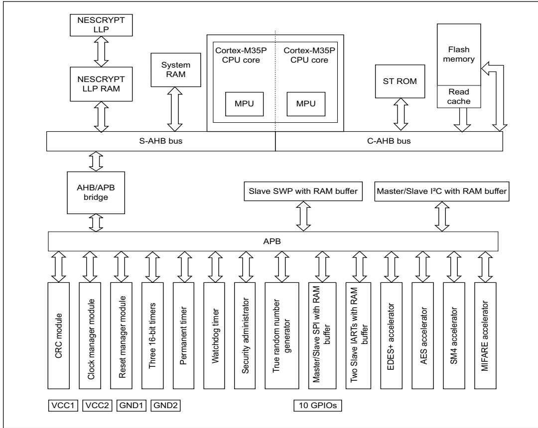
Figure 1. ST33K1M5A and ST33K1M5M B03 block diagram
