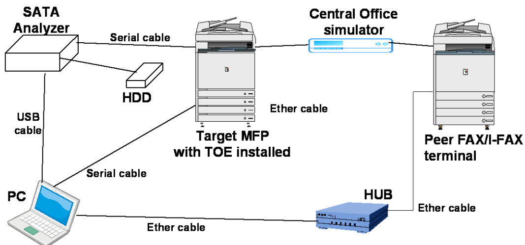
Figure 2-1: Developer test configuration
