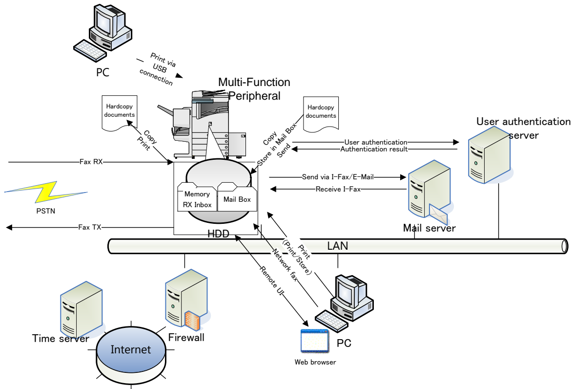
Figure 1 The assumed operational environment of the MFP < Canon imageRUNNER ADVANCE 45900KG/4500 Series >
