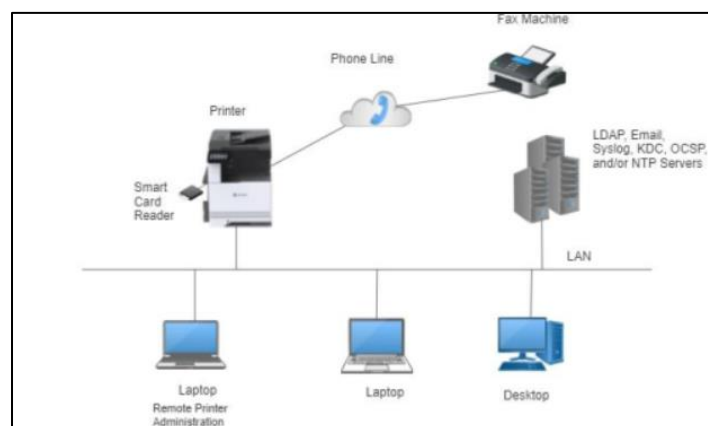
Figure 1: TOE Architecture
