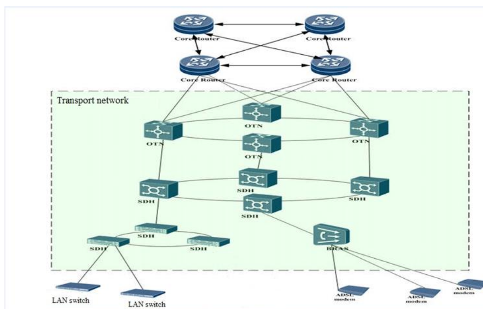
Figure 1-1 Position of the transmission network on the entire communication network
