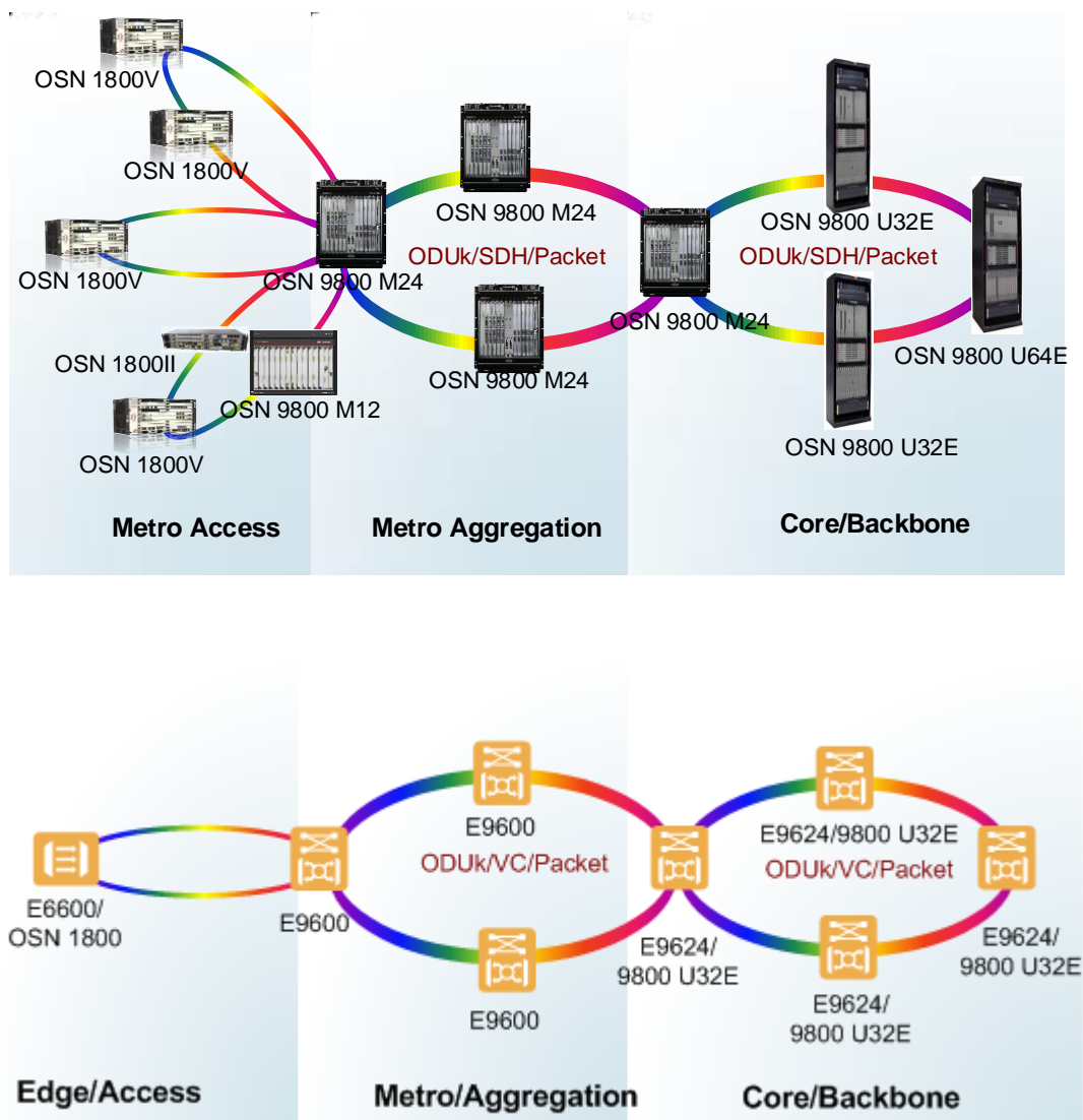
Figure 1-2 Position of the OptiX OSN 1800 OptiXtrans E6608T/E6608/E6616, on the entire network
