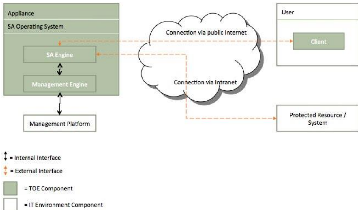
Figure 1 – TOE Boundary
