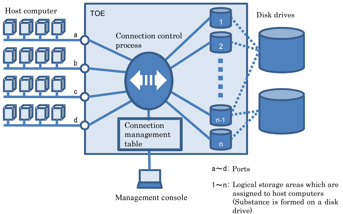
Figure 1-3 Connection control between host computers and logical storage areas
