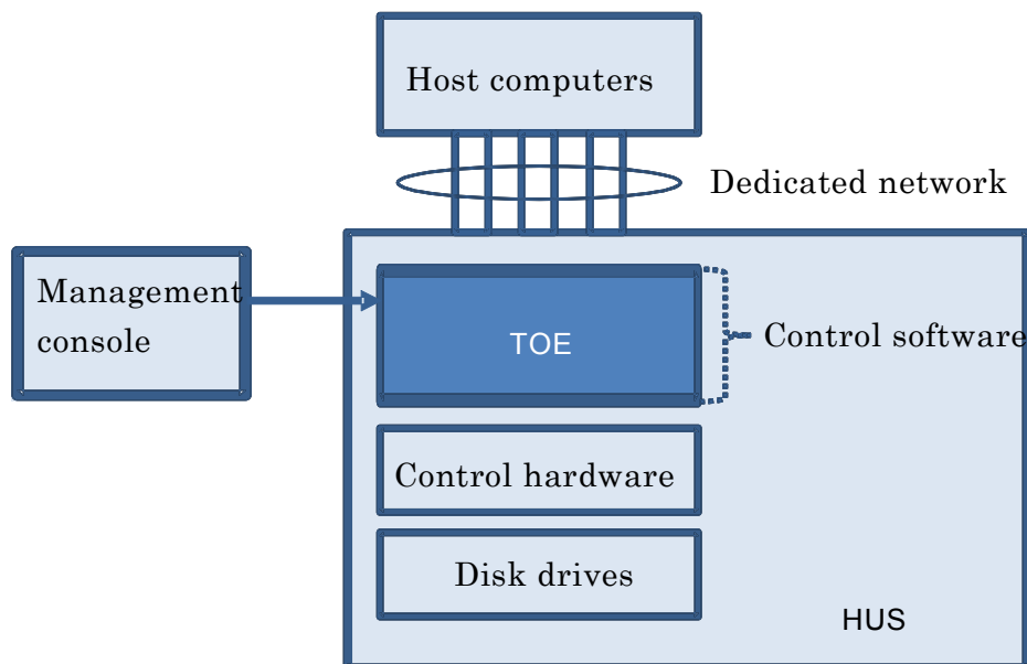
Figure 1-2 TOE and its IT environment
