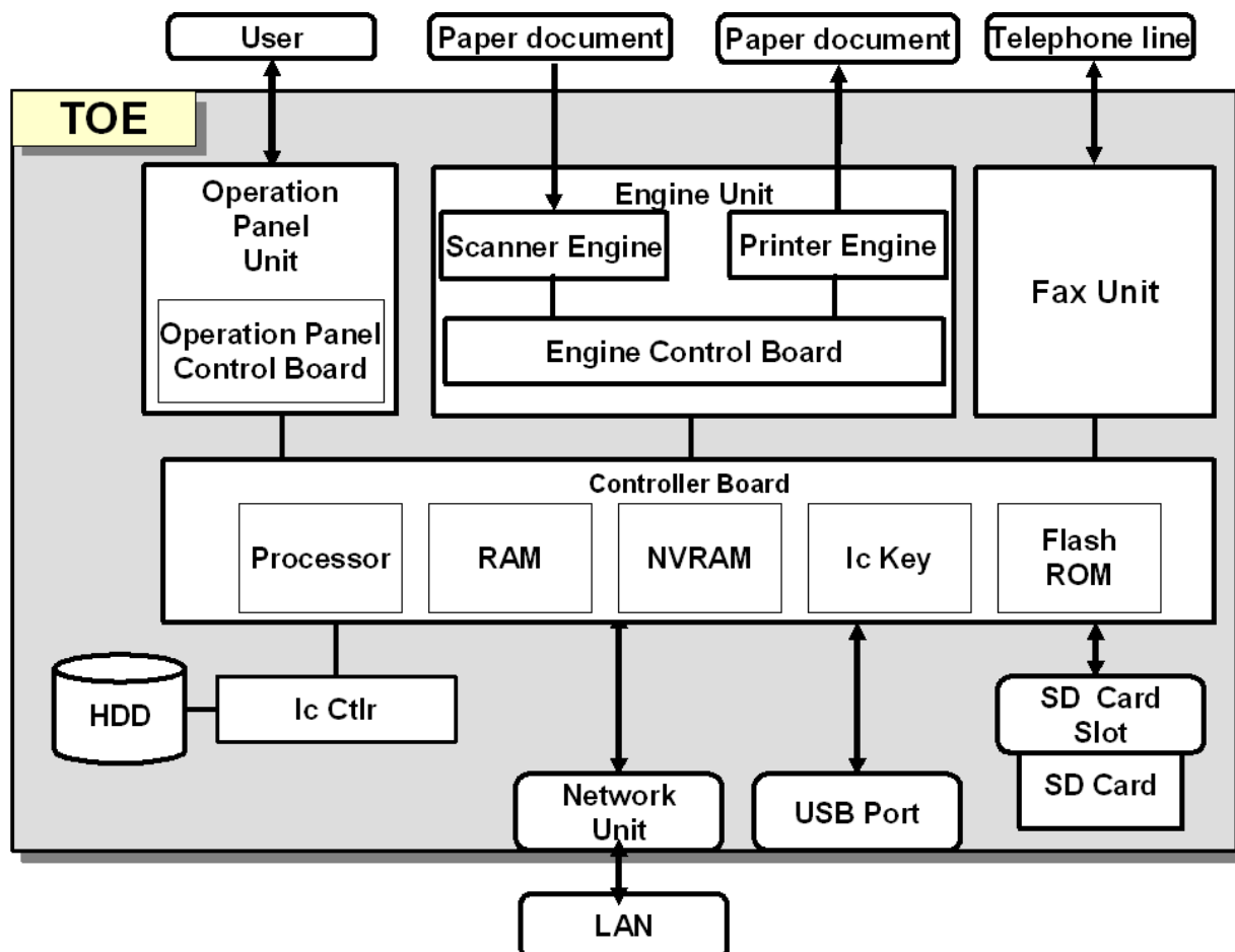
Figure 5-1 TOE boundary
