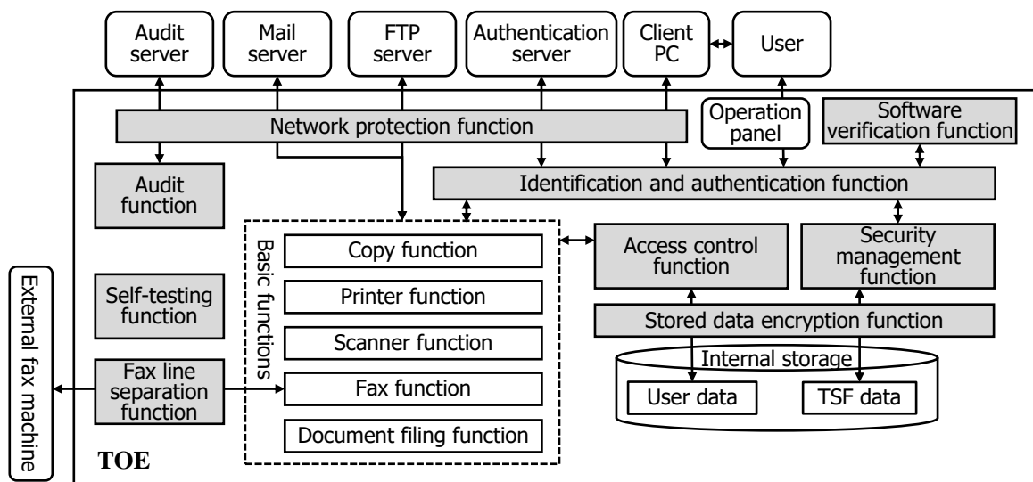
Figure 5-1 TOE boundary
