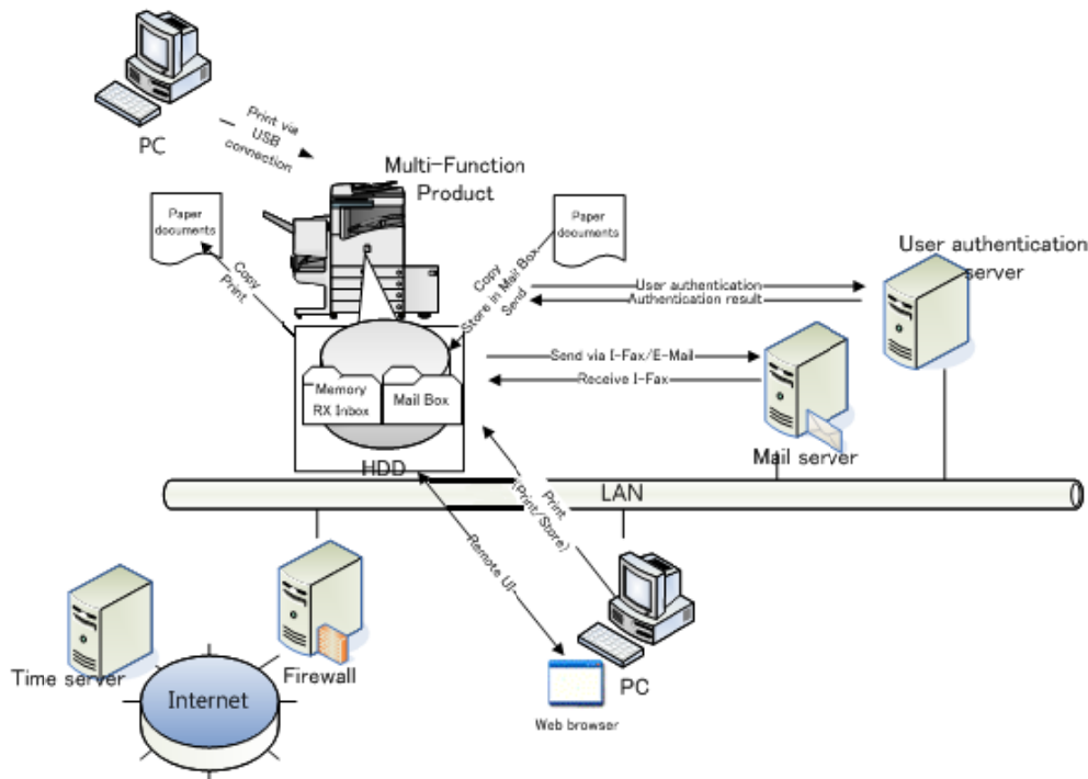
Figure 1 The assumed operational environment of the MFP < Canon imagePRESS C800/C700/C700L/C600 >
