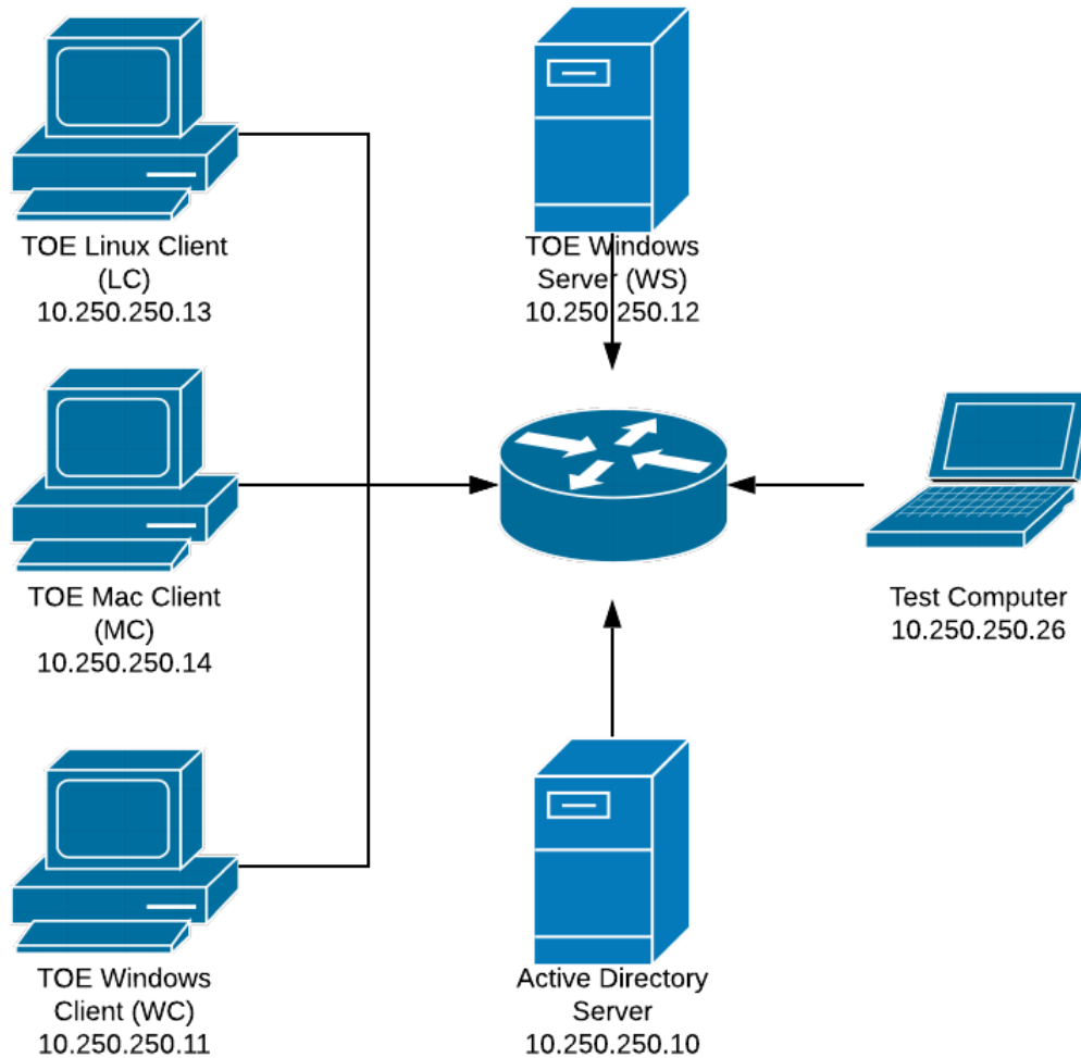
Figure 2 Test Configuration
