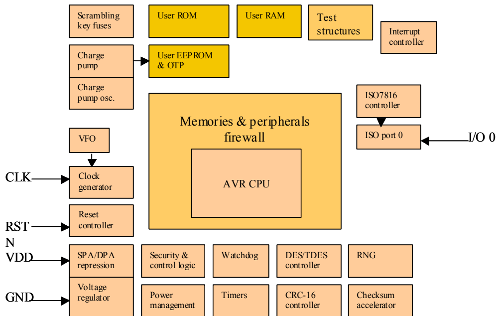
Figure 1 - micro-circuit ATMEL AT90SC6404RT
