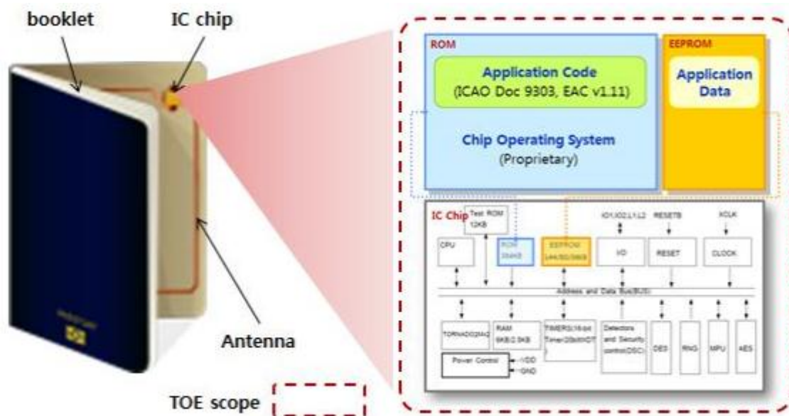
[Figure 2]Physical boundary of the TOE
