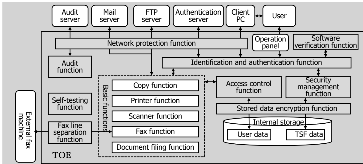
Figure 5-1 TOE boundary
