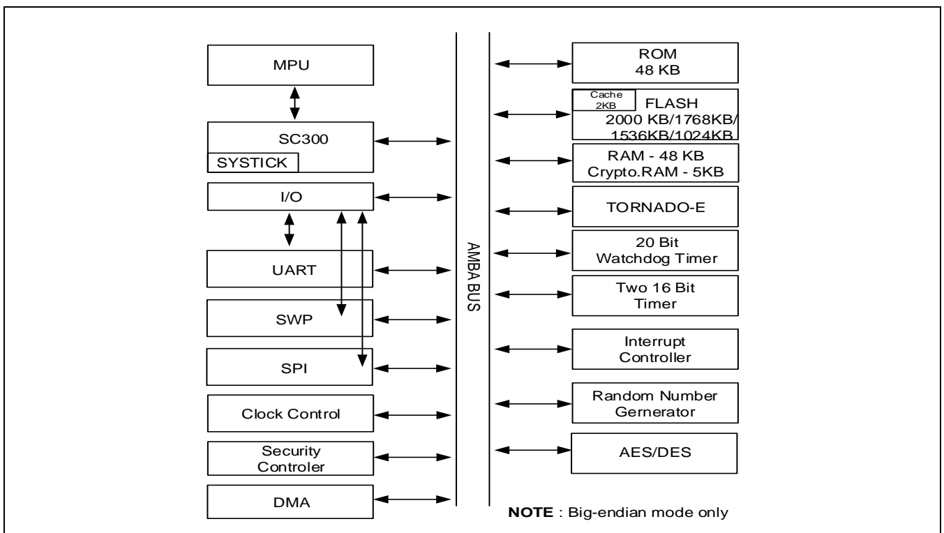
Figure 1 S3FV9RR/S3FV9RQ/S3FV9RP/S3FV9RK Block Diagram
