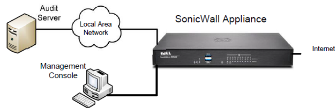
Figure 1 TOE Architecture
